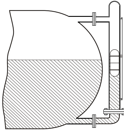
STYLE A1L (ANGLE PIPE)
